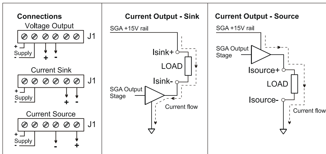
Figure 2.5 Output Connections
